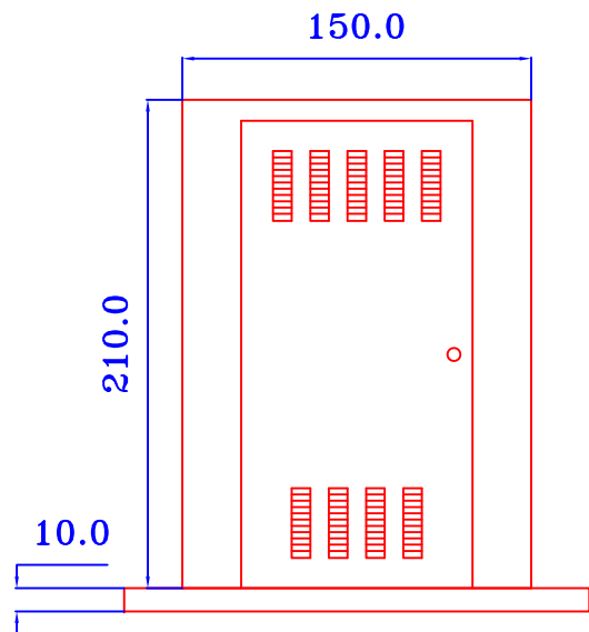
ALZADO PRINCIPAL
